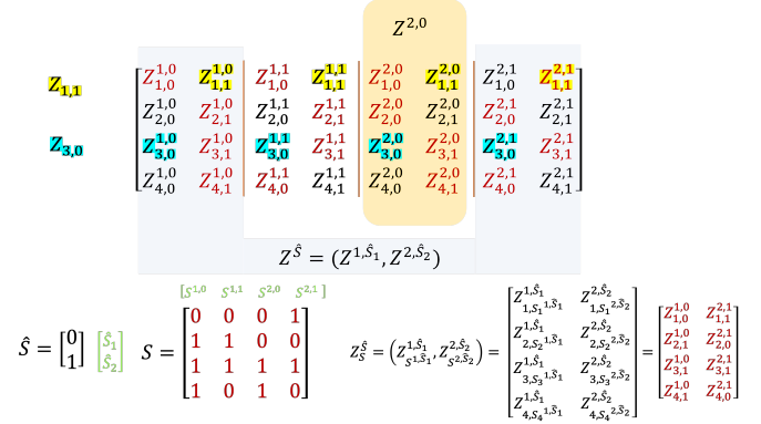
Fig. 2. A graphical representation of the notation system. We chose m = 2 , i.e., 4 meta tasks, and n = 4 , i.e., 8 data samples per task.
